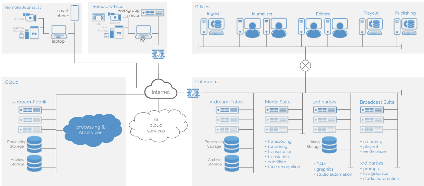
x-dream-Fabrik hybrid deployment
